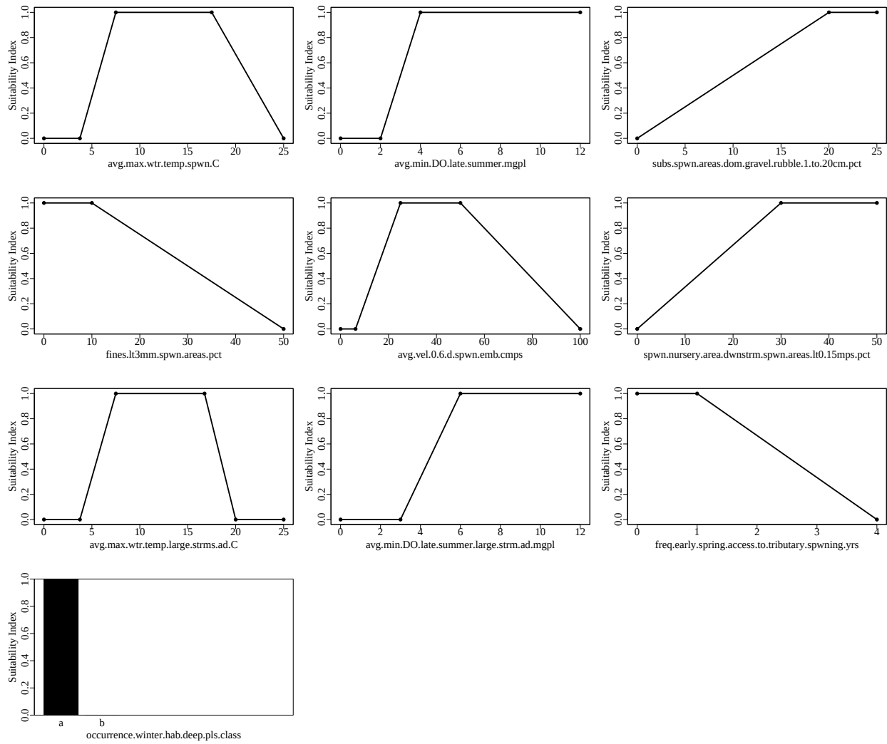
Figure 1. Suitability index graphs for variables included in the arcticgrayling model in ecoest.
